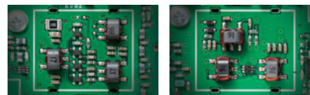
HF/50 MHz Quad Mixer
