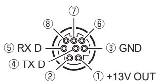
TUNER/LINEAR Jack
