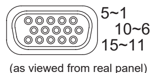
CONTROL I/O connector
